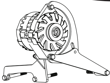
ASSEMBLED VIEW
